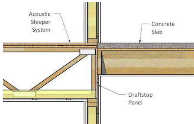
Figure 4: Section at non-bearing partition
