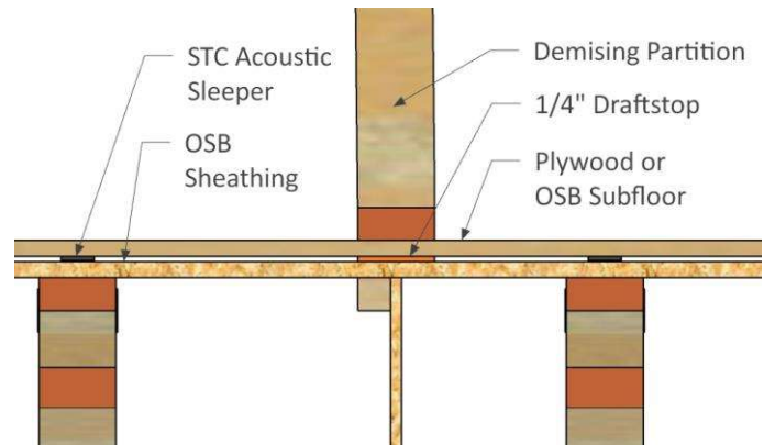
Figure 5: Typical section at Breezeway
